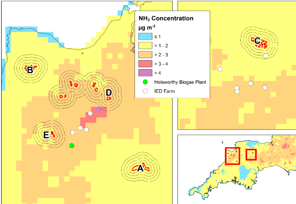
Figure 3: Ammonia concentrations at Culm Grasslands SAC (FRAME 1 km dataset for 2011), showing the location of IED farms and a biogas plant surrounding the site
