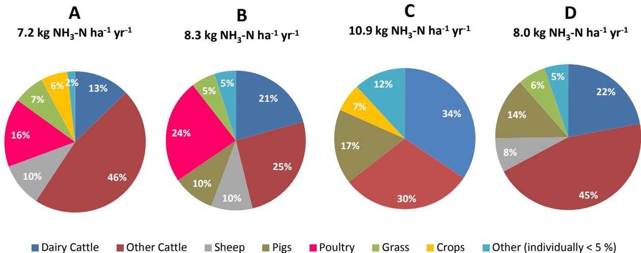
Figure 6: Agricultural NH 3 emission sources in the 2km zone surrounding the sub-sites of North York Moors derived from 2012 agricultural census and their corresponding emission densities
